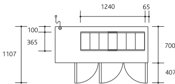
Integral top view
