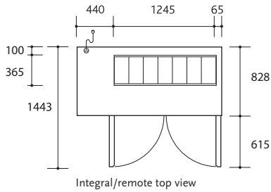
Integral/remote top view
