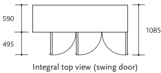
Integral top view (swing door)
