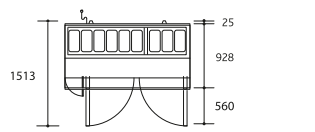
Integral top view
