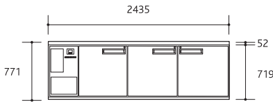
Integral/remote front elevation
