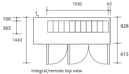
Integral/remote top view
