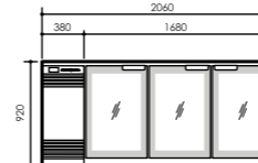
Integral front elevation
