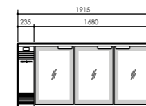
Remote front elevation
