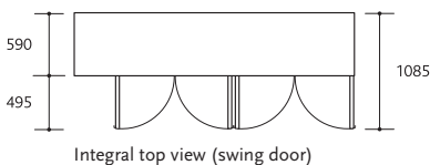
Integral top view (swing door)
