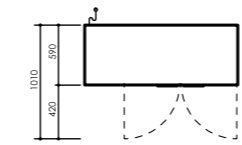
Integral top view
